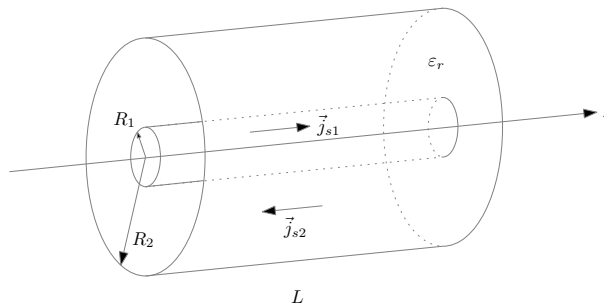
FIGURE 61 – Câble coaxial
