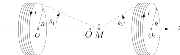
FIGURE 53 – Bobines en configuration Anti-Helmholtz
